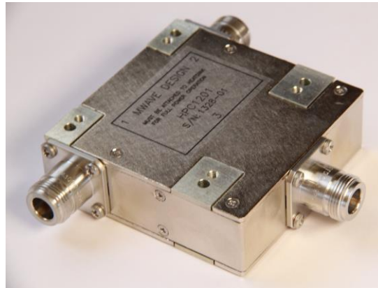
VHF Band 2 Kw Circulator
